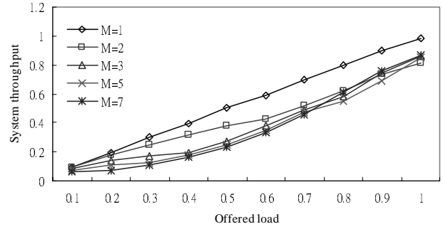
Fig. 9. System throughput for different fixed number of assigned PDCHs to an MS.
