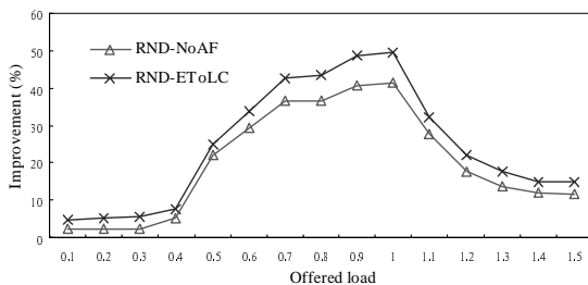
Fig. 7. Improvement in system throughput for proposed load-balancing schemes over the RND-RND scheme.
