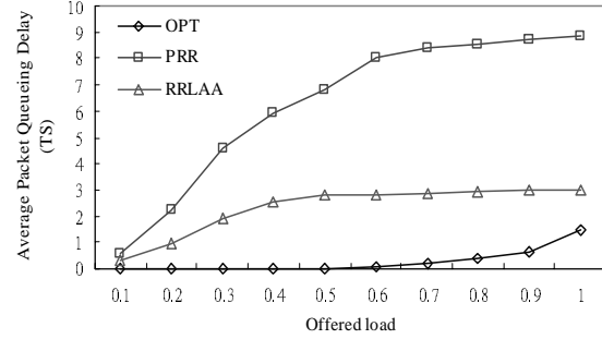
Fig. 12. Average packet queuing delay for different selection schemes.
