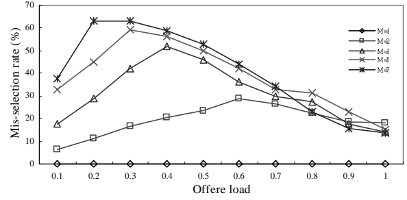
Fig. 8. Mis-selection rates for different fixed number of assigned PDCHs to an MS.
