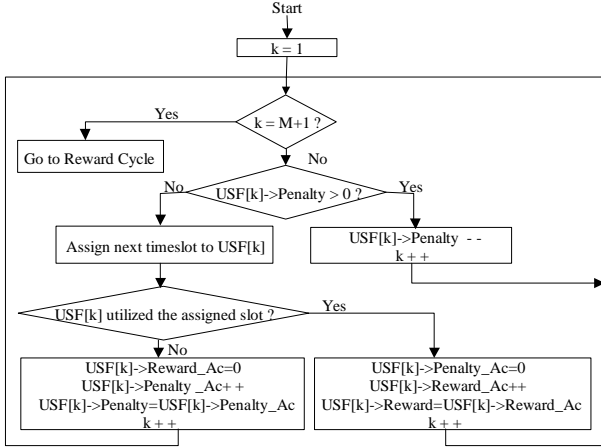
Fig. 2. The procedure to process a Penalty cycle.
