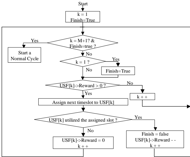
Fig. 3. The procedure to process a Reward cycle.
